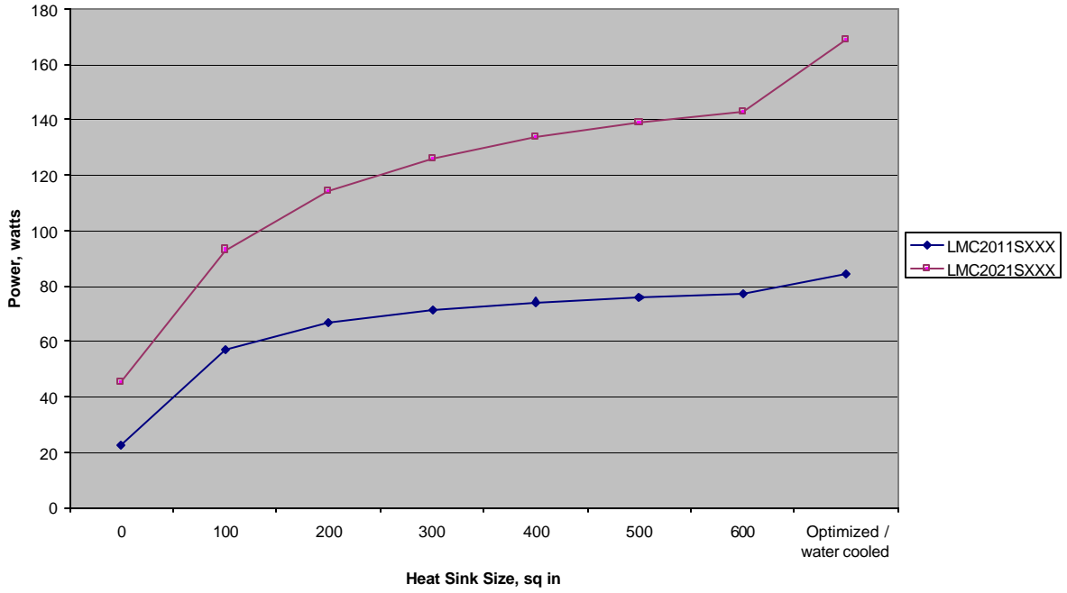
2000 LM Max Power vs Heat Sink Size For a 100°C temperature rise (Maximum operating temperature is 125°C)
